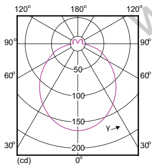
CLA LEDspotMV ND 5W PAR16 GU10 830 520lm
